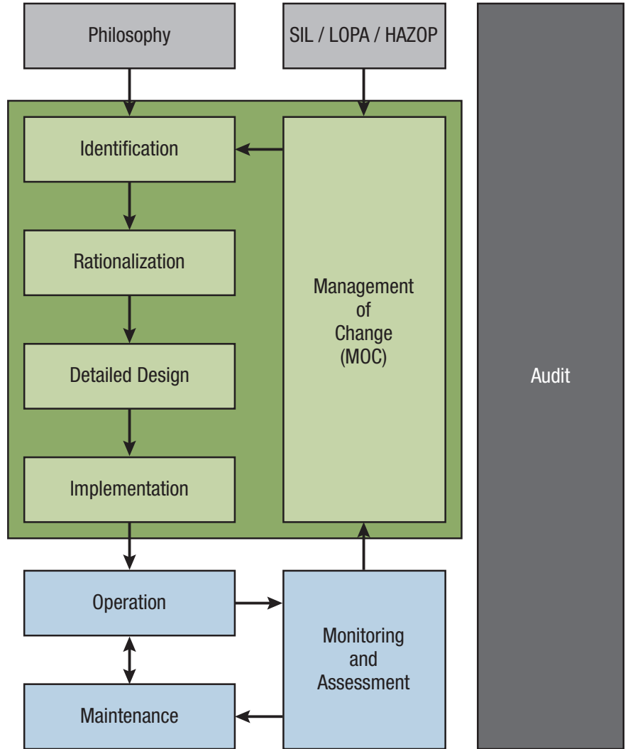
Figure 1 – OESuite™ models the entire ISA 18.2 Alarm Management lifecycle
